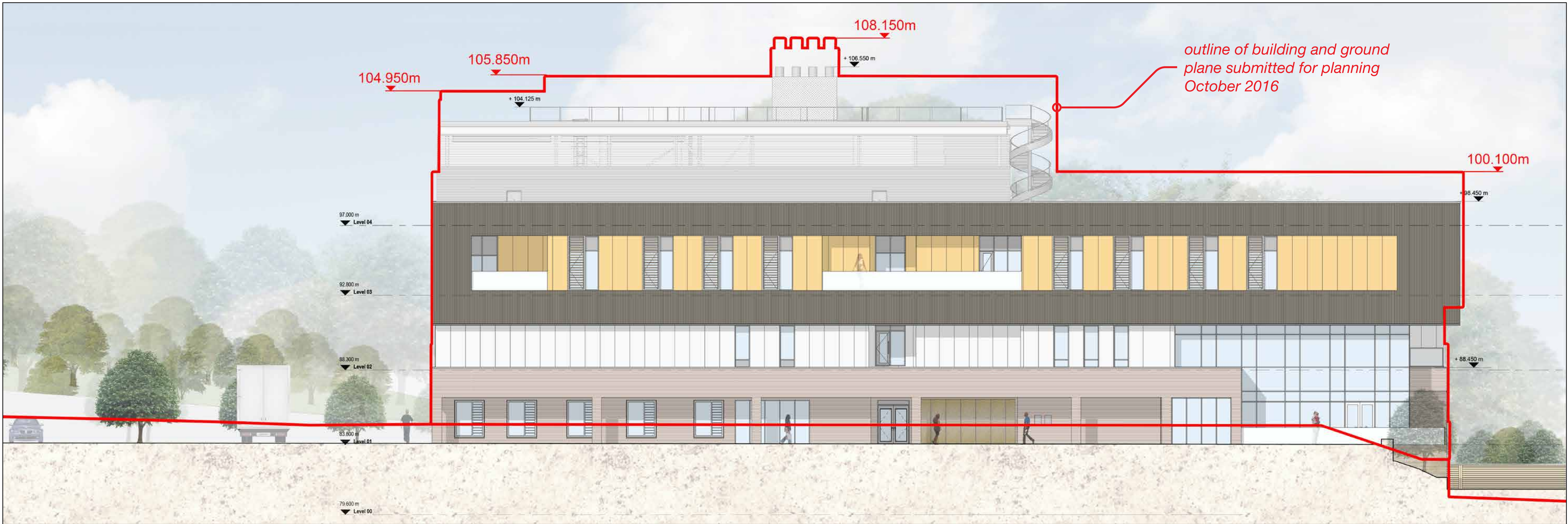
Southwest Elevation: April 2017
